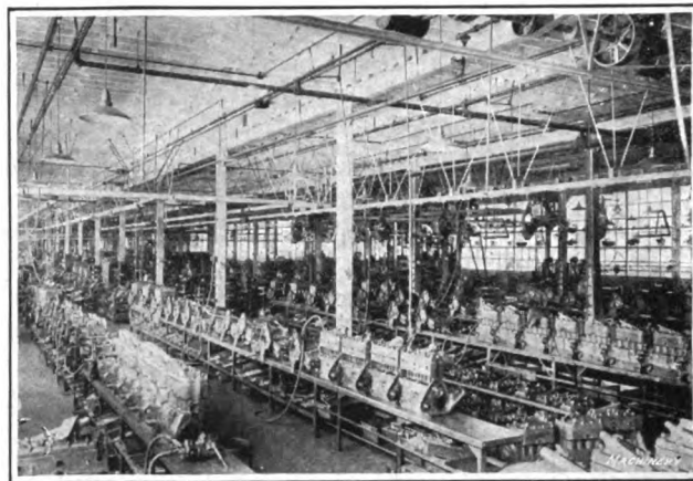
Fig. 24—Overhead conveyors are used in the motor assembling department of the Willys-Overland Co., Toledo, O., for carrying the larger parts of the motors to the assembling benches. Small parts are held in New Britain tote boxes underneath the benches, where they are within convenient reach of the operator
